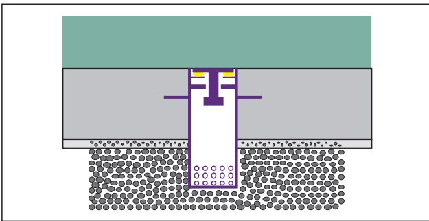
Groundwater flap valve KA 6
