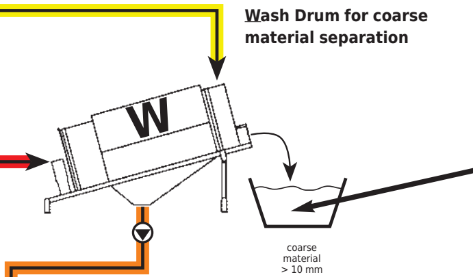
ROTAMAT® Wash Drum for washout and separation of all coarse material > 10 mm
