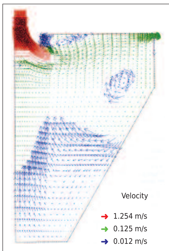
Flow velocities in the COANDA Grit Washing Plant RoSF 4 (measured by TU Munich)
