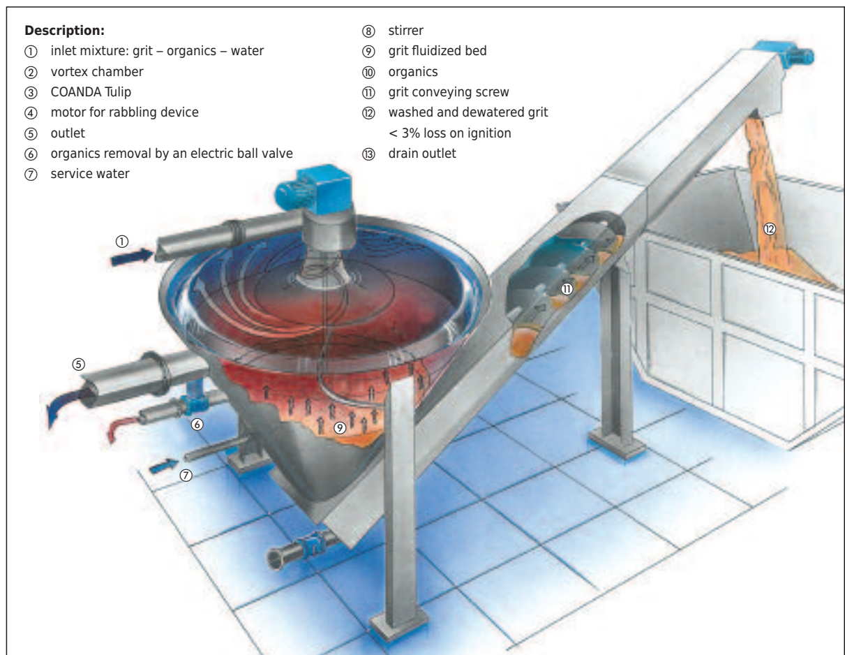
Flow diagram of a COANDA Grit Washing Plant RoSF 4
